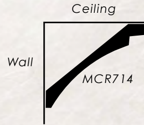
Projection: 5-1/2" Height: 4-5/8"
