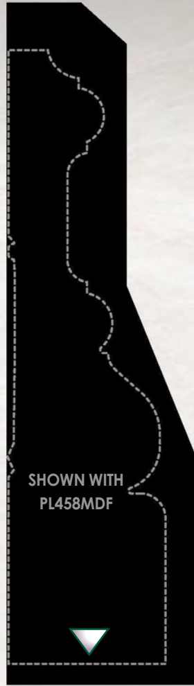
PB518 1-7/16 x 5-1/8 Will accommodate all casings and most casing/backband combinations 4" to 4-7/8" in width
