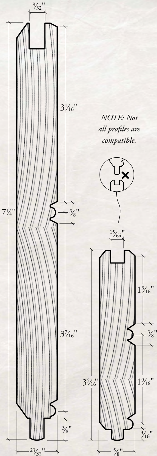
SPBC8 standard T&G beadboard 16'
